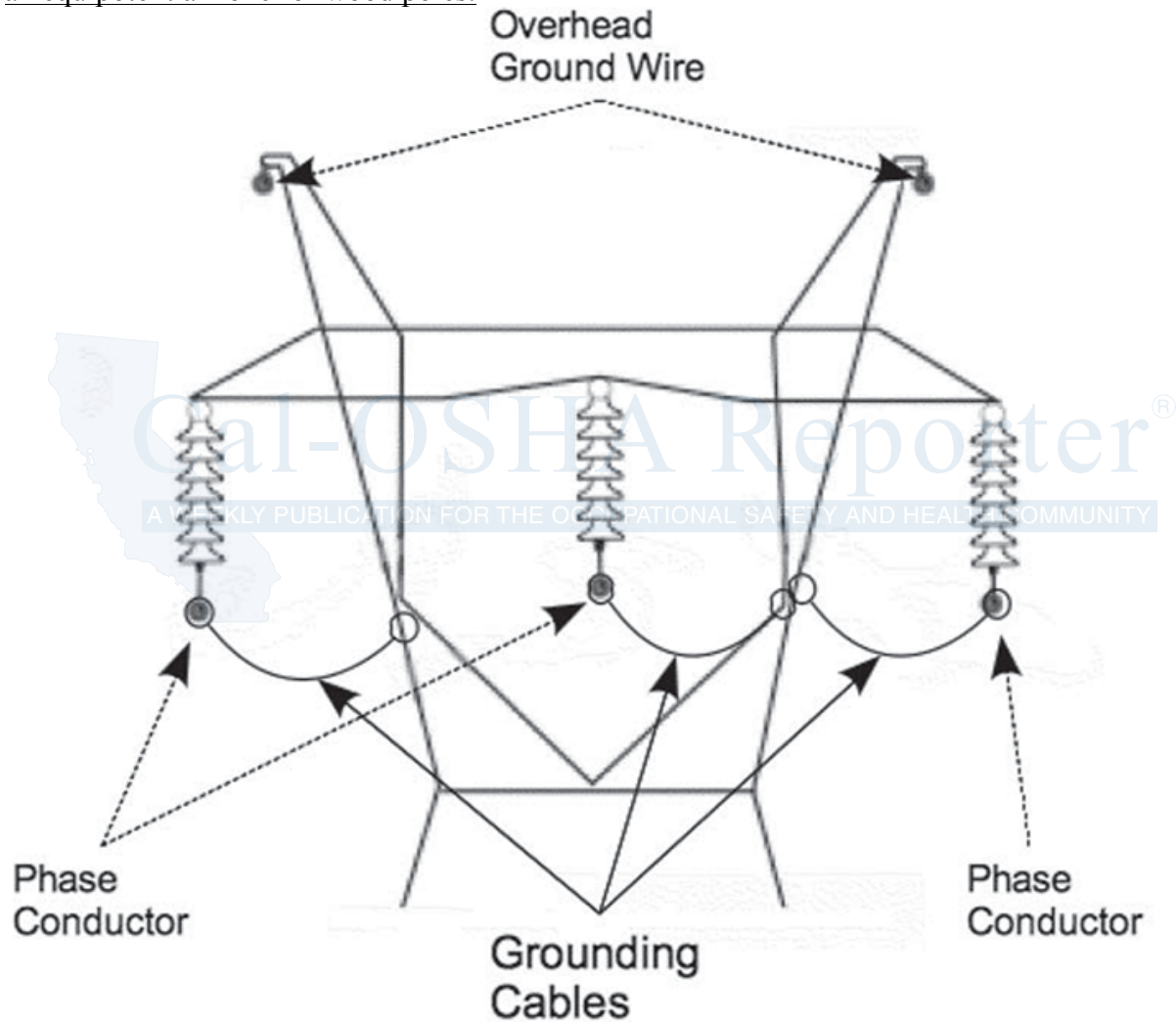
Figure 4 - Equipotential Zone for Metal Lattice Tower
