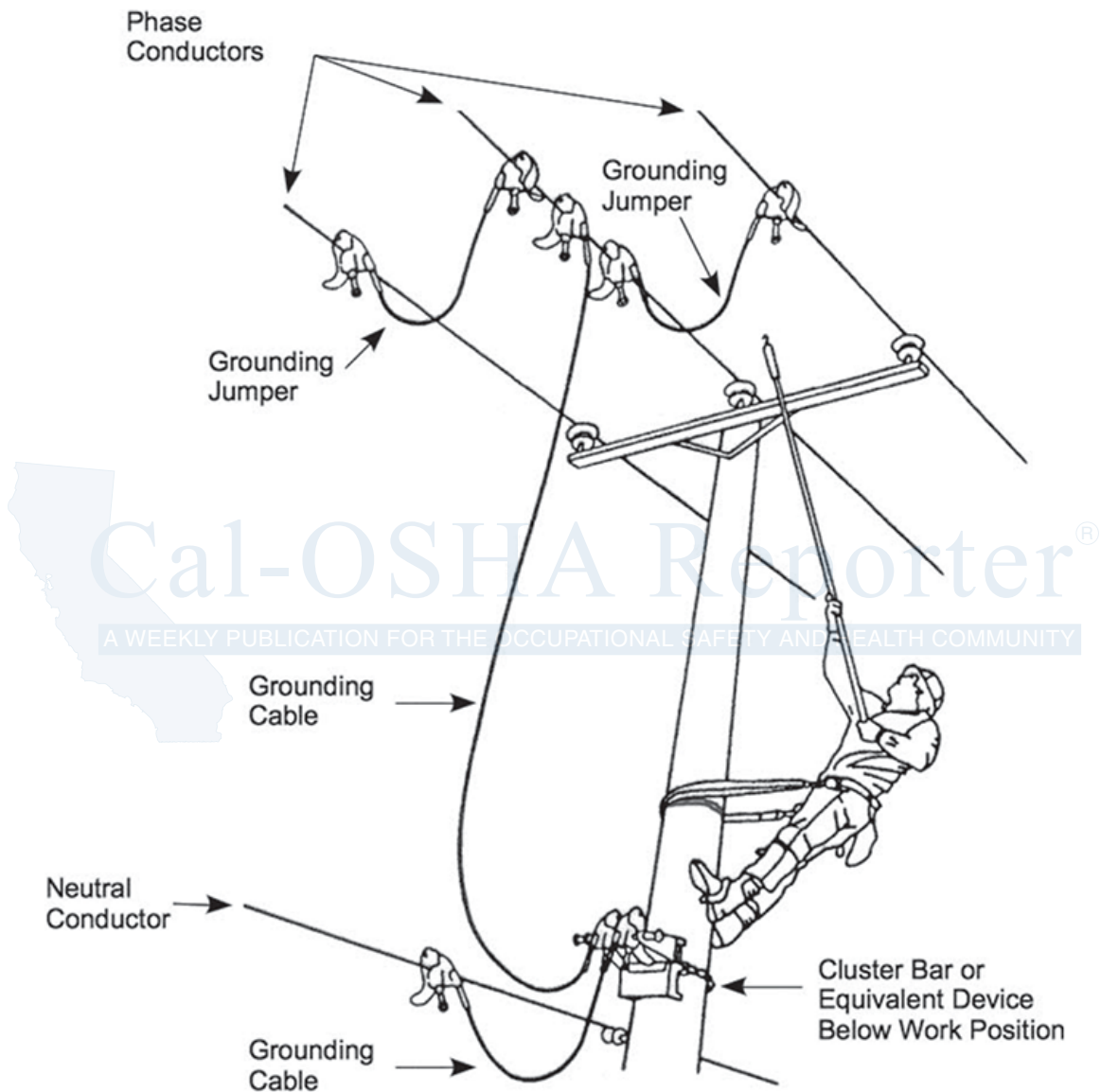
Figure 5 - Equipotential Grounding for Wood Poles
