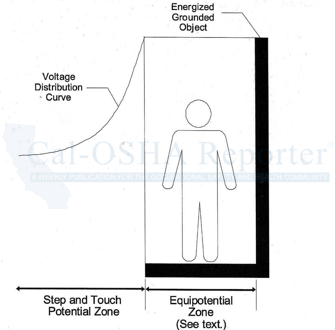
Figure 3—Protection from Ground-Potential Gradients
